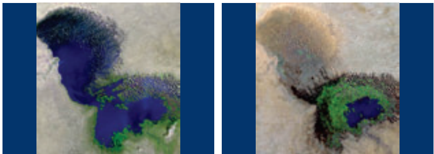
Picture: satellite photos of Lake Chad in 1972 (left) and 1987 (right).
